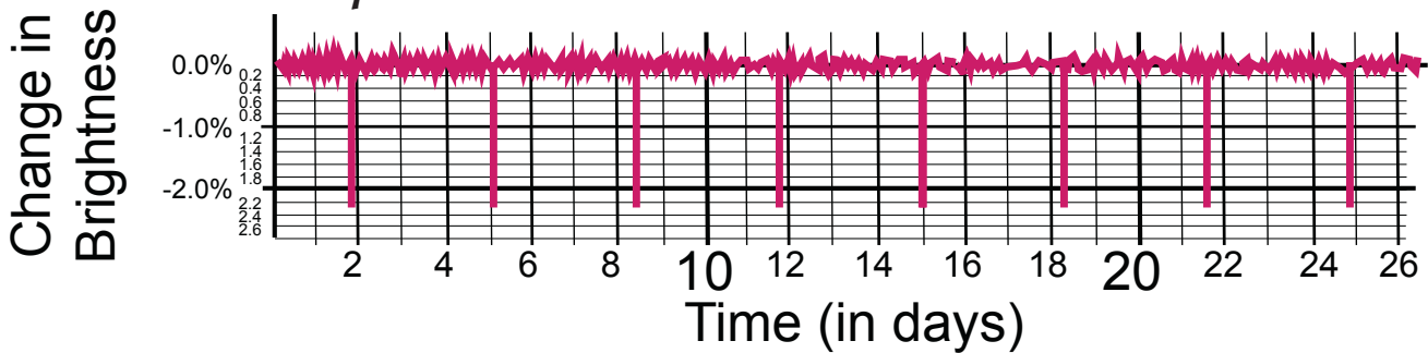
Kepler 7b
