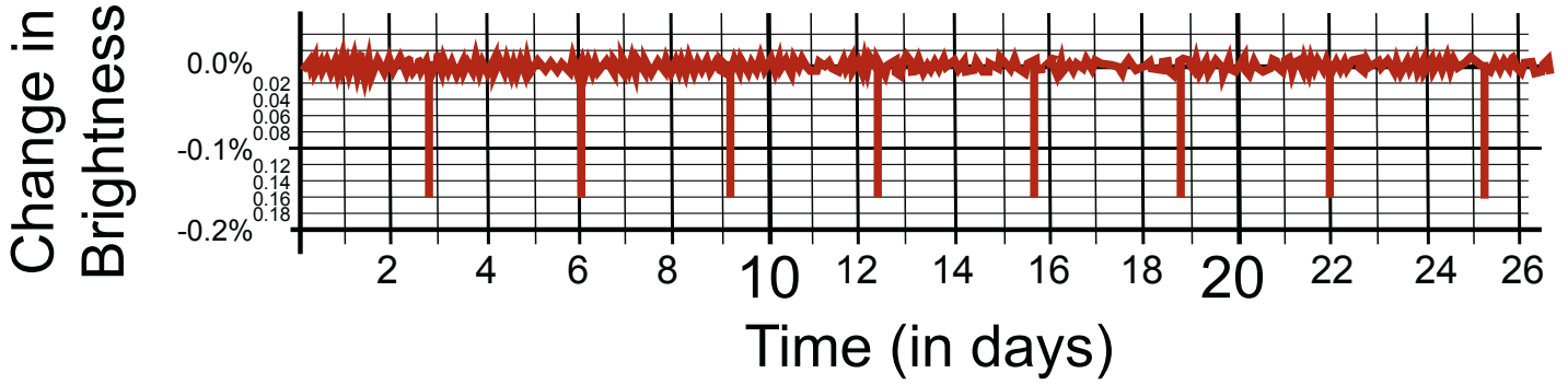
Kepler 4b
