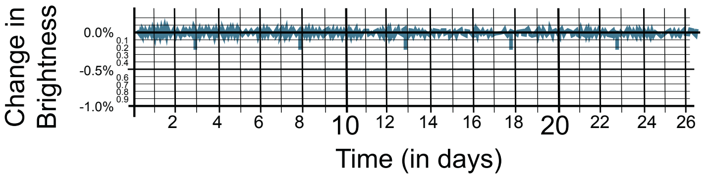
HAT-P-11b
