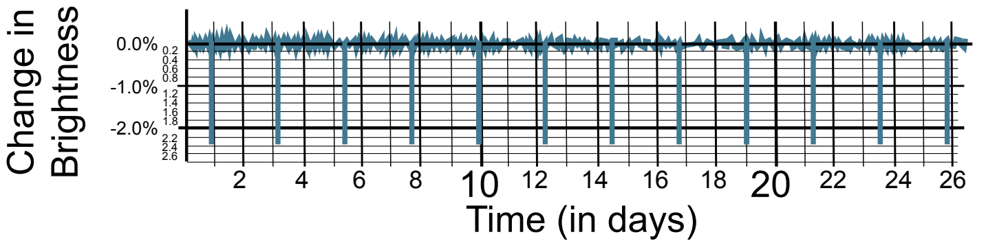
HAT-P-7b
