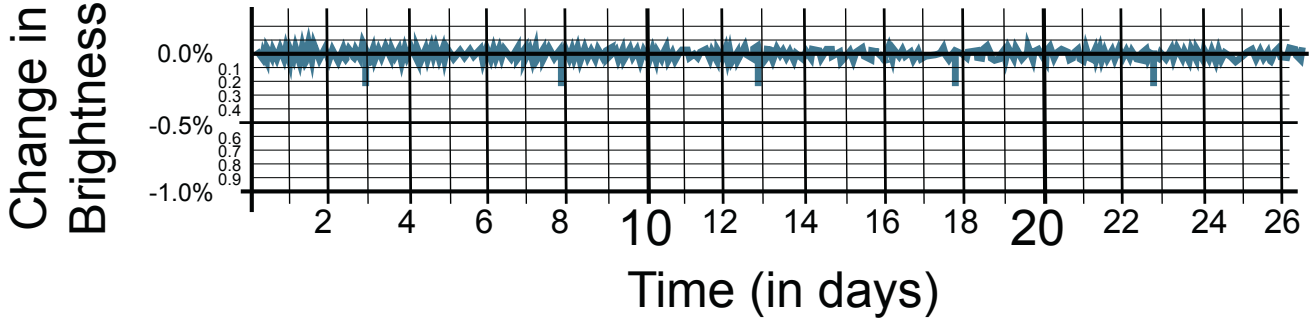
Kepler 5b
