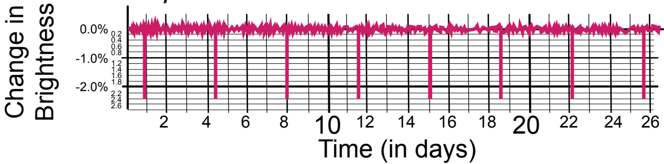
Kepler 6b
