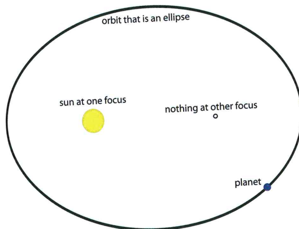
Figure 2-14: Diagram related to Kepler's first law.
