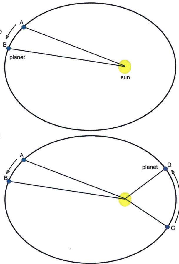
Figure 2-15: Diagrams related to Kepler's second law
